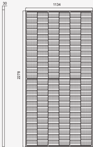
Vista Frontal
